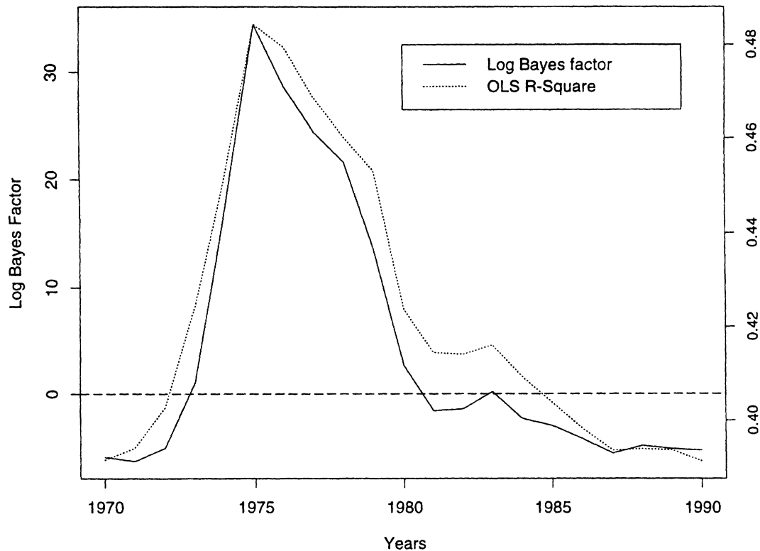
Figure 1. Log Bayes factors and OLS R^2 statistics from a model of a structural break in the determinants of real growth.
